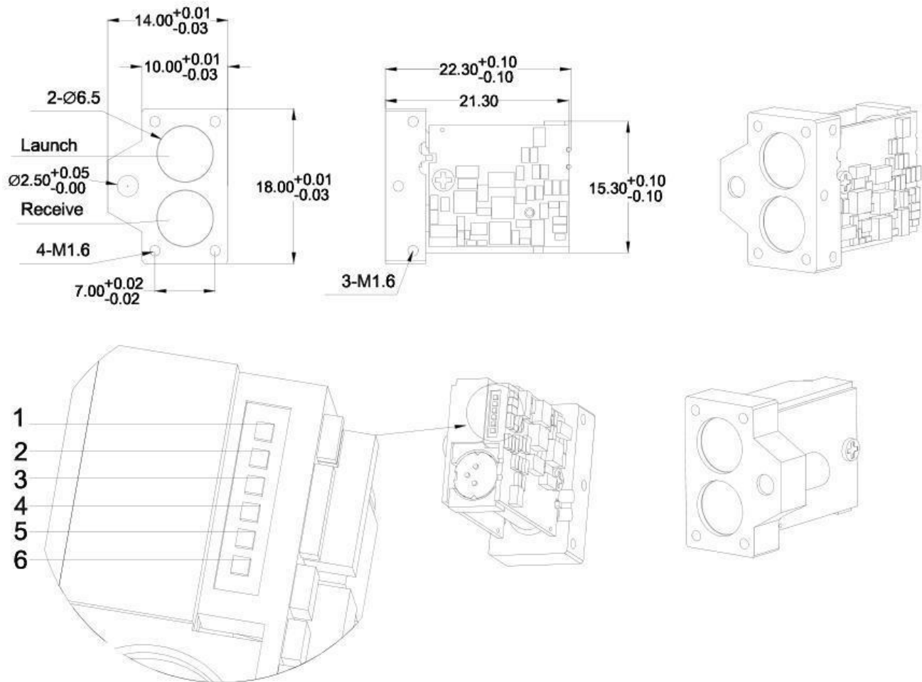
Figure 1 SPD1200N3 Mechanical Drawing and Electrical Interface (mm)
